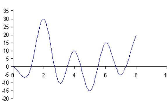
Figure A.1 Typical segment of a stress history
