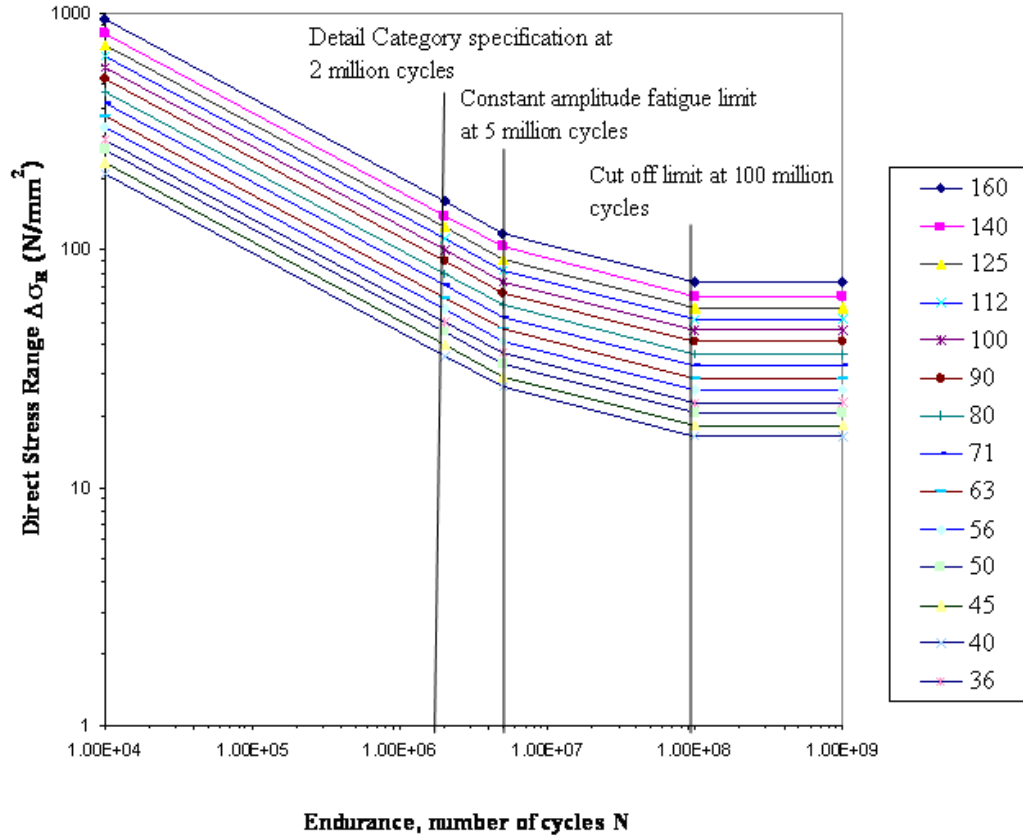
Figure 10.2: Fatigue Strength curves for normal stress ranges
