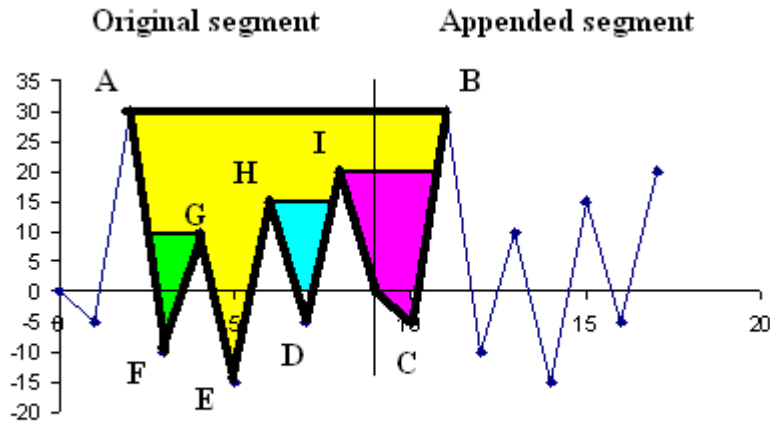
Figure A.4 Drainage sequence from troughs of the reservoir
