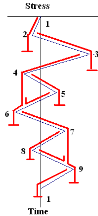
Figure A.7 Rainflow patterns
