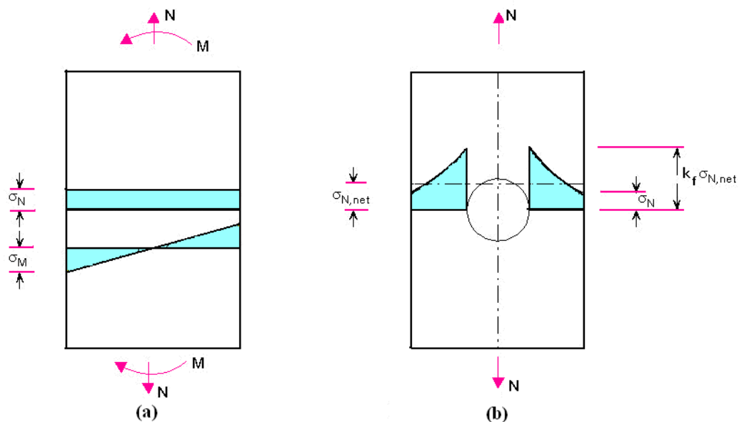
Figure-11.1 Nomination stress and geometric stress concentration
