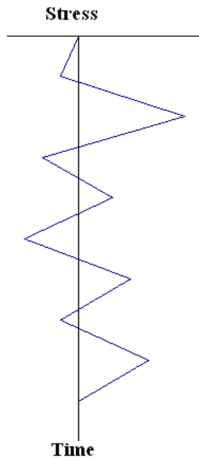
Figure A.6 Rotation of axes for rainflow counting
