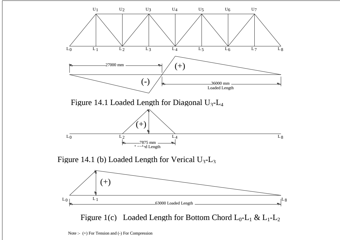
Figure 14.1: Loaded lengths for finding \lambda_1 .
