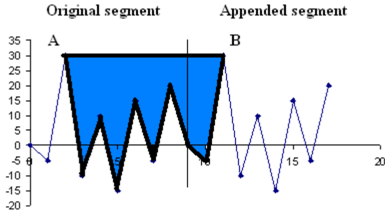
Figure A.3 Original and appended stress history
