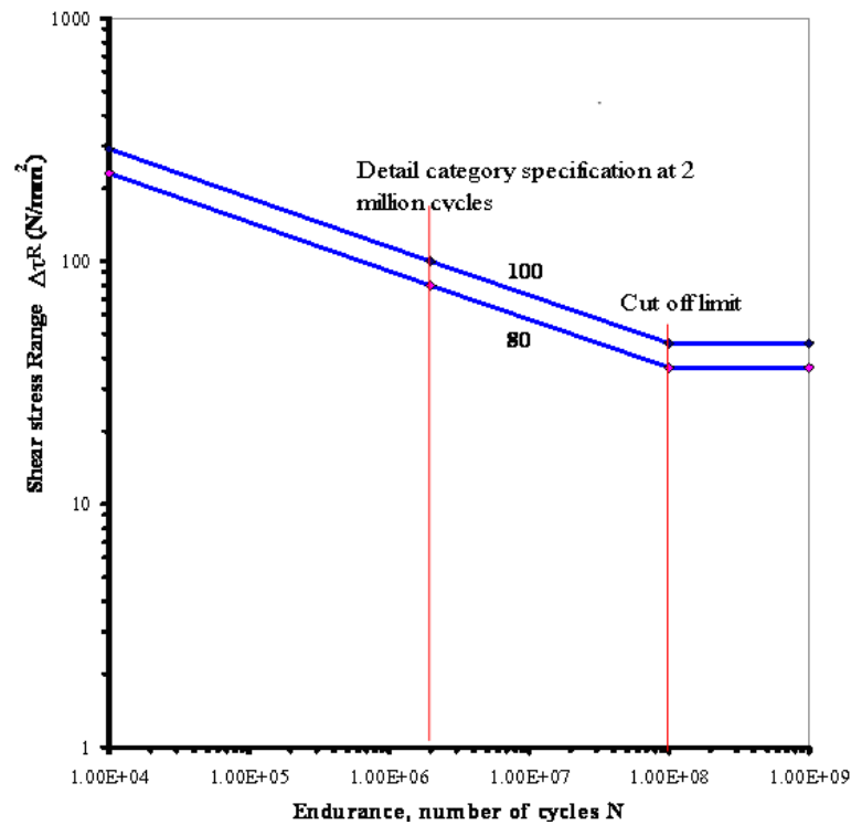
Figure 10.3: Fatigue Strength curves for shear stress ranges
