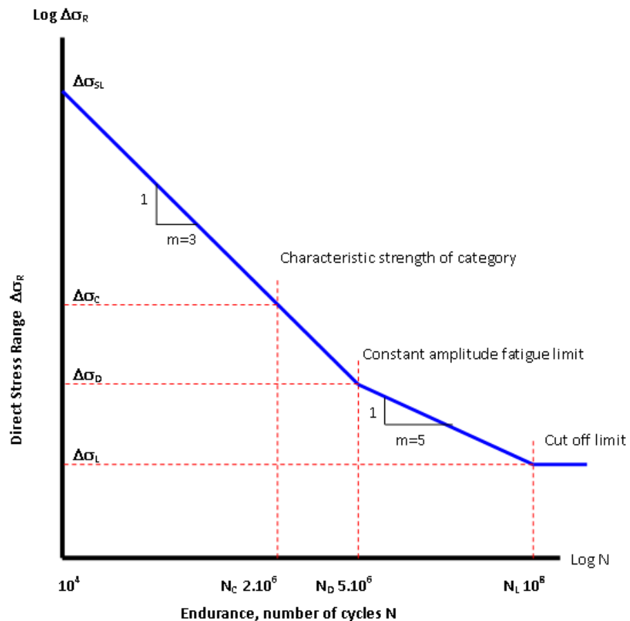
Figure 10.1: Typical fatigue strength (S-N) curve
