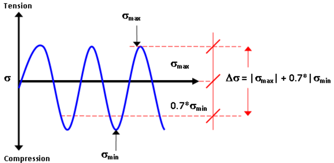
Figure 10.4: Modified stress range for non-welded or stress relieved details
