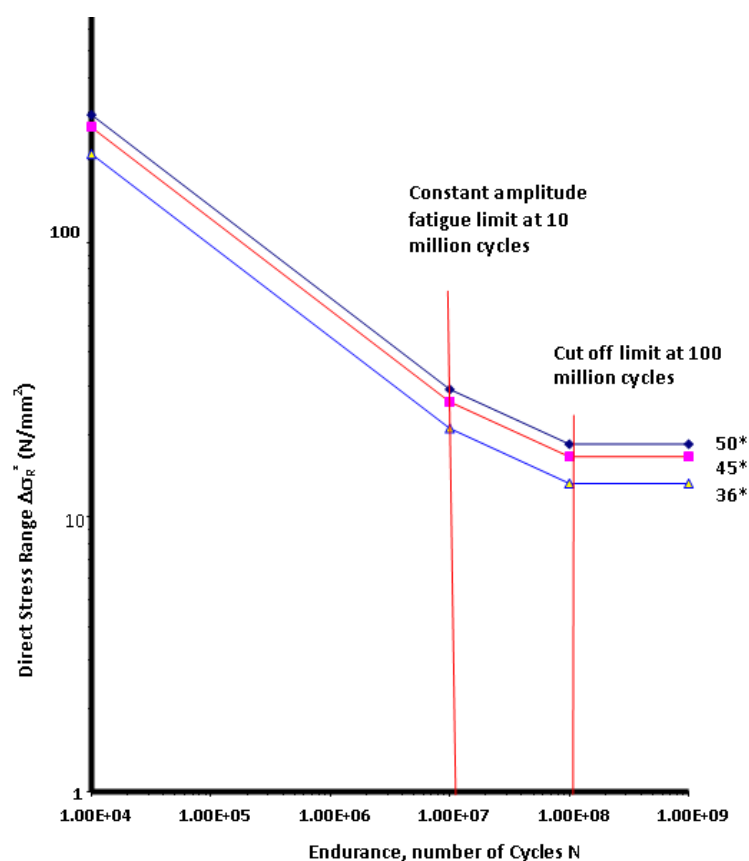
Figure 10.5: Modified fatigue Strength Curves
