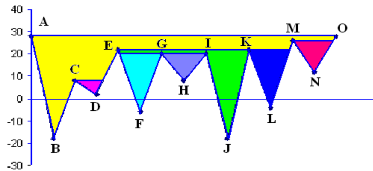
Figure A.5 Reservoir section showing drainage sequence
