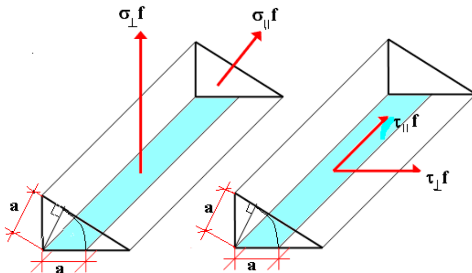
Figure-11.2 stresses in fillet welds
